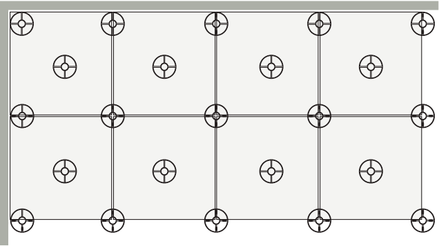
Posa sopraelevata 60x60 \pm 2 cm 24"x24" \pm \frac{3}{4} " Installation onto flat surfaces (raised laying)
