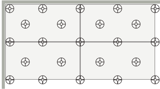
Posa sopraelevata 60x90 \pm 2 cm 24"x36" \pm \frac{3}{4} " Installation onto flat surfaces (raised laying)
